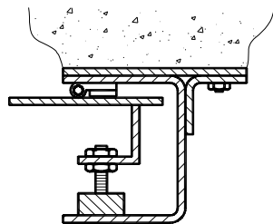
FRAME DETAIL
